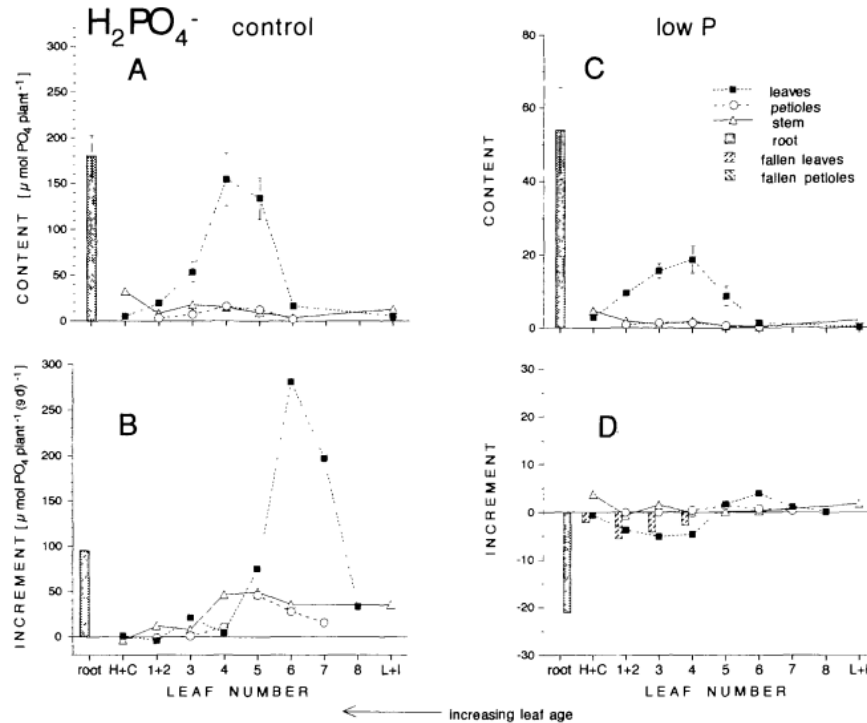
Figure 4: Effect of Low and high P application on stem and leaves Andrews 1985.
