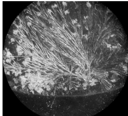
Figure 3. Real "bouquets of flowers" are formed in drying \text{NaCl} solutions prepared in negatively charged water [30].
