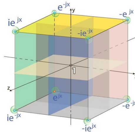
Figure 3: Model of a qubit with embedded cubits.
