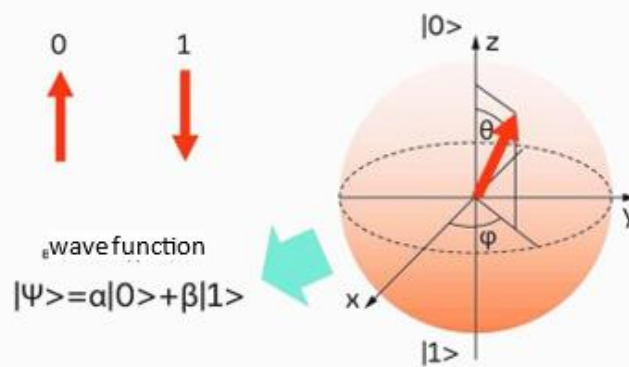
Figure 4: "Bloch Sphere" as a qubit model.
