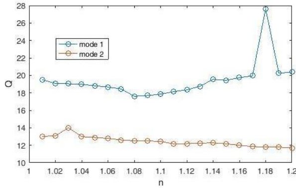
Figure 7: Quality factor diagram of Q plasmonic sensor.
