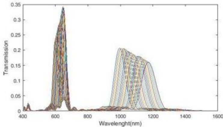
Figure 3: Transmission spectra of plasmonic refractive index sensor.
