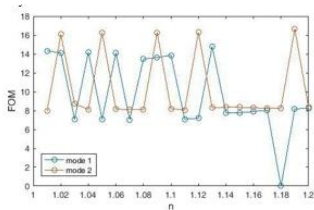
Figure 6: Plasmonic sensor FOM competency diagram.
