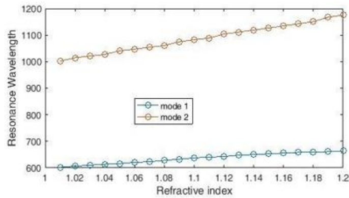
Figure 4: Resonance wavelength versus refractive index analysis.
