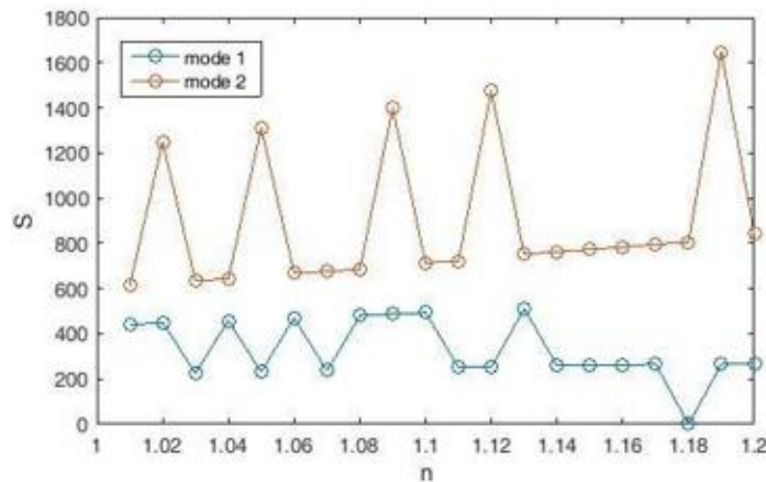
Figure 5: Plasmonic sensor sensitivity coefficient diagram.
