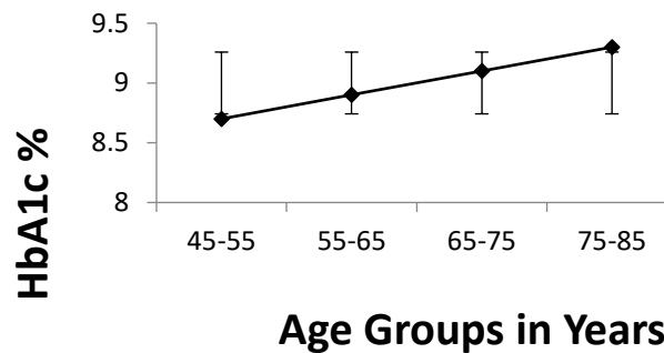
Figure 1: Relationship between HbA1c of different age groups shown with error bars. Regression coefficient, r = 0.387
