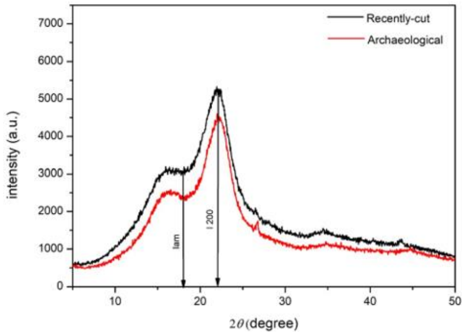
Figure 3: X-ray diffractograms from archaeological and recently-cut oak.
