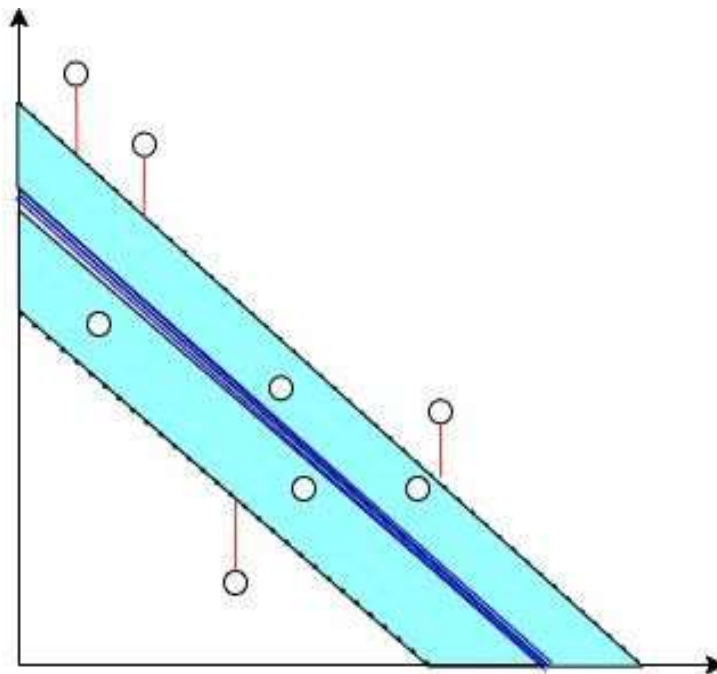
Figure 6. Support vector regression diagram
