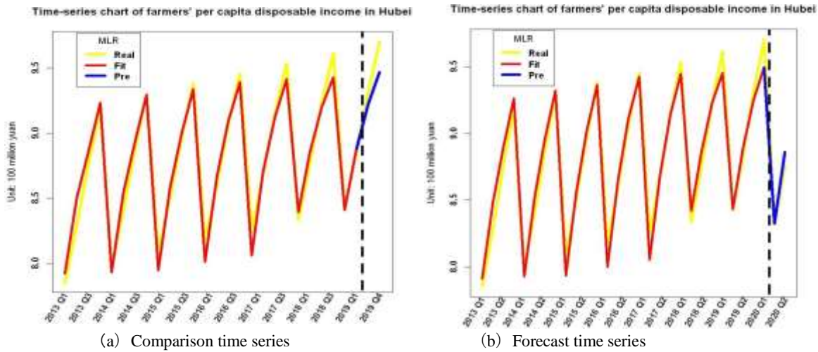
Figure 5. Comparison and prediction sequence diagram of multiple linear regression models
