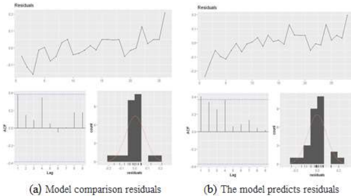
Figure 7: Model comparison with forecast residual graph
