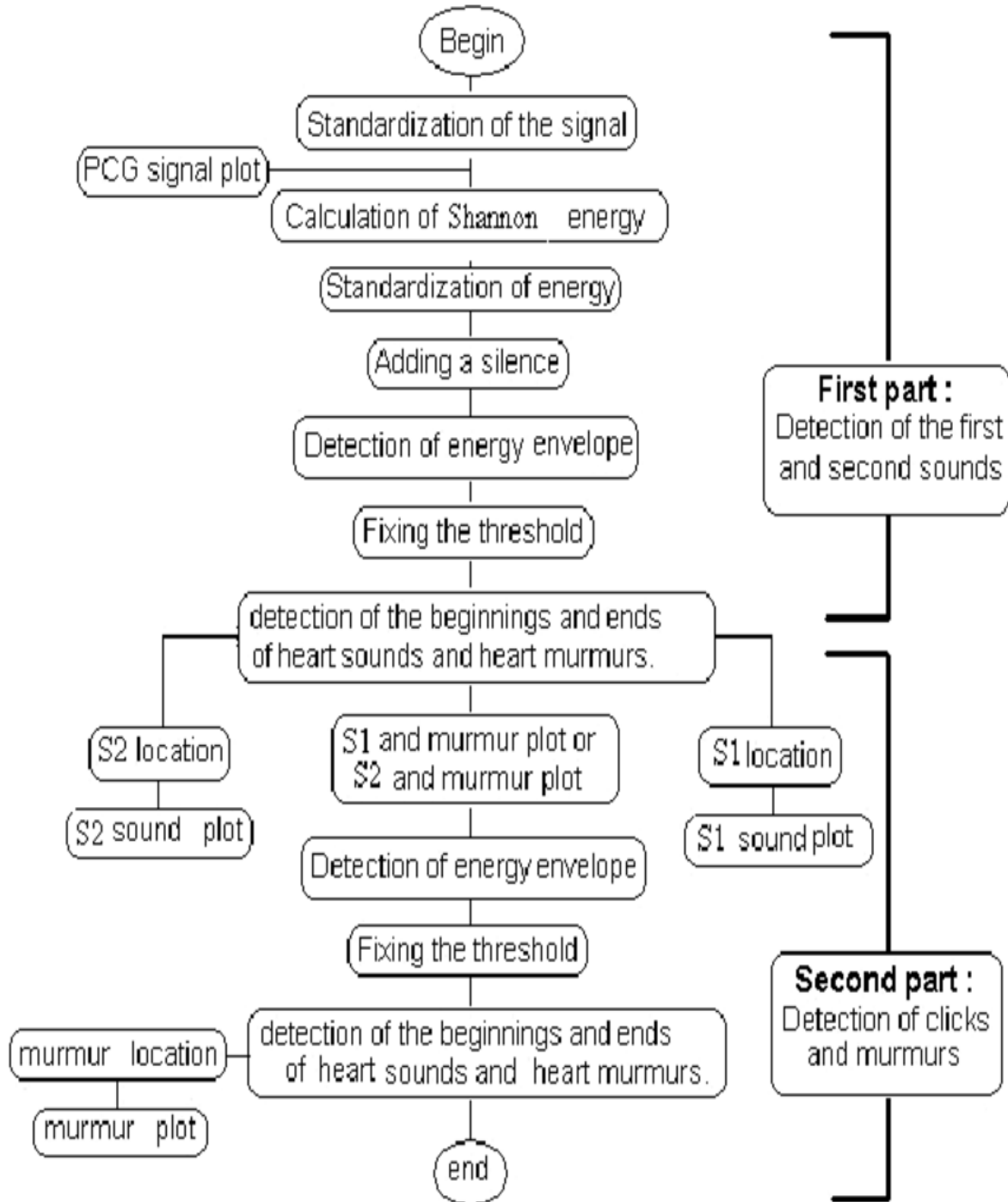
Figure 3: separation algorithm
