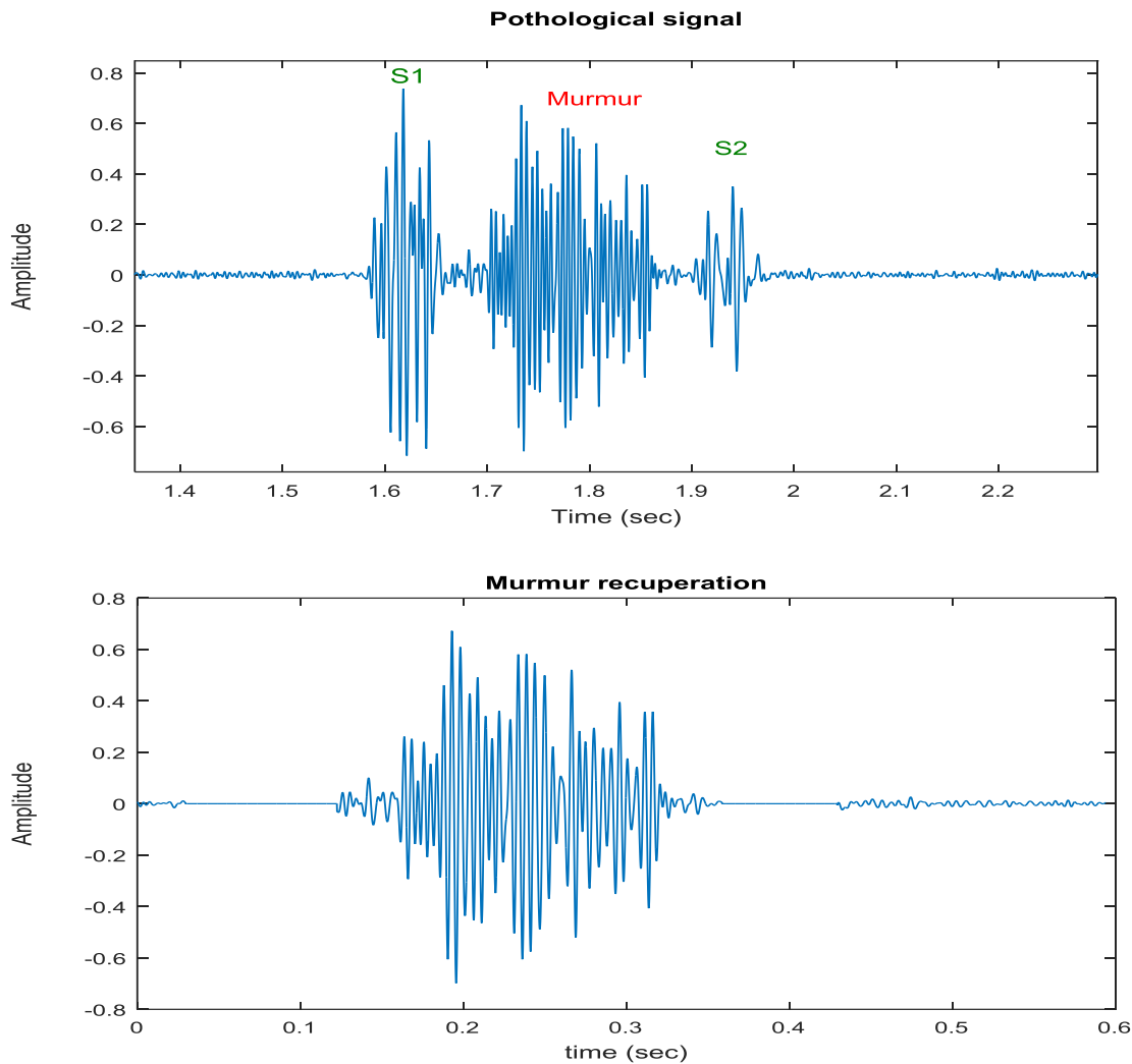
Figure 4: Murmur extraction
